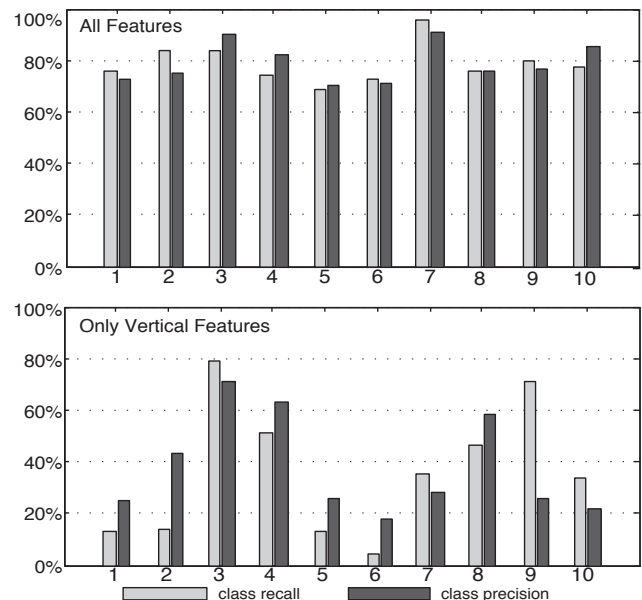
Figure 2: The figure shows the class precision and class recall for each of the classes (see text for explanation). A class consists of sound-tracings related to the same sound. High scores on both bars indicate that the estimation of this class is satisfactory. In the top chart, all features have been used as input to the classifier, in the lower chart, only the vertical displacement features were used.
